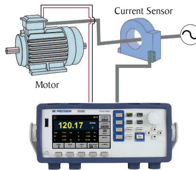
Power Meter
